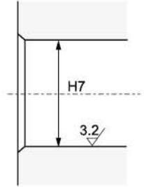
Mating Housing 相配座孔
