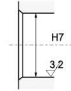
Mating Housing 相配座孔
